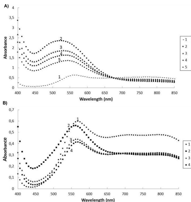
Figure 2. Solutions of [V IV (HIDPA) 2 ] 2- (A) or [V IV (HIDA) 2 ] 2- (B, concentrations 0.02 M), before and after treatment with Ce 4+ (pH ca. 1). A) 1, before addition of Ce 4+ ; 2, 5 min after addition of ca. 1 equiv Ce 4+ relative to the vanadium complex; 3, 2 h 30 min; 4, 4 h; 5, 6 h; 6, 20 h (identical to 1). B) 1, before addition of Ce 4+ ; 2, 7 min after addition of ca. 1 equiv Ce 4+ relative to the complex; 3, 9 min; 4, 12 min.
